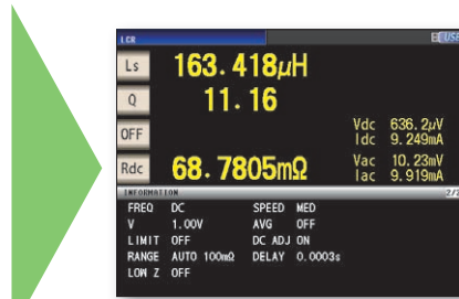
L/Q (1 kHz, 1 mA constant current measurement) and DCR (DC measurement) display screen
