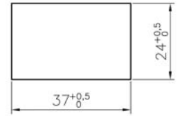
Panel cut-out
