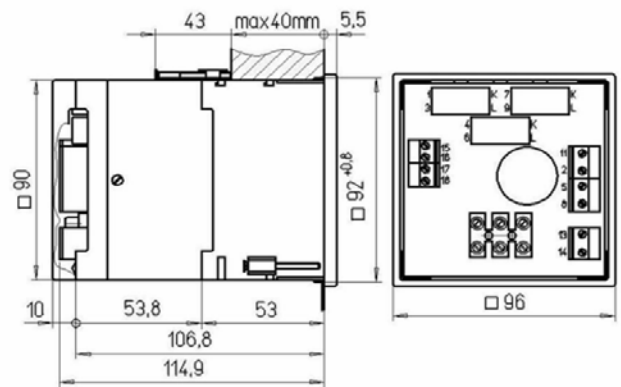
Picture 3: Dimensional drawing (all dimensions are in mm)
