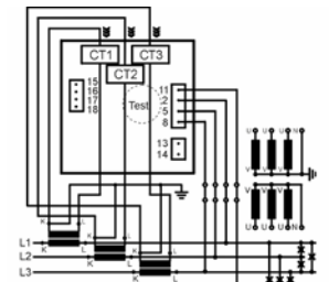
Picture 7: Three-phase connection (4u)
